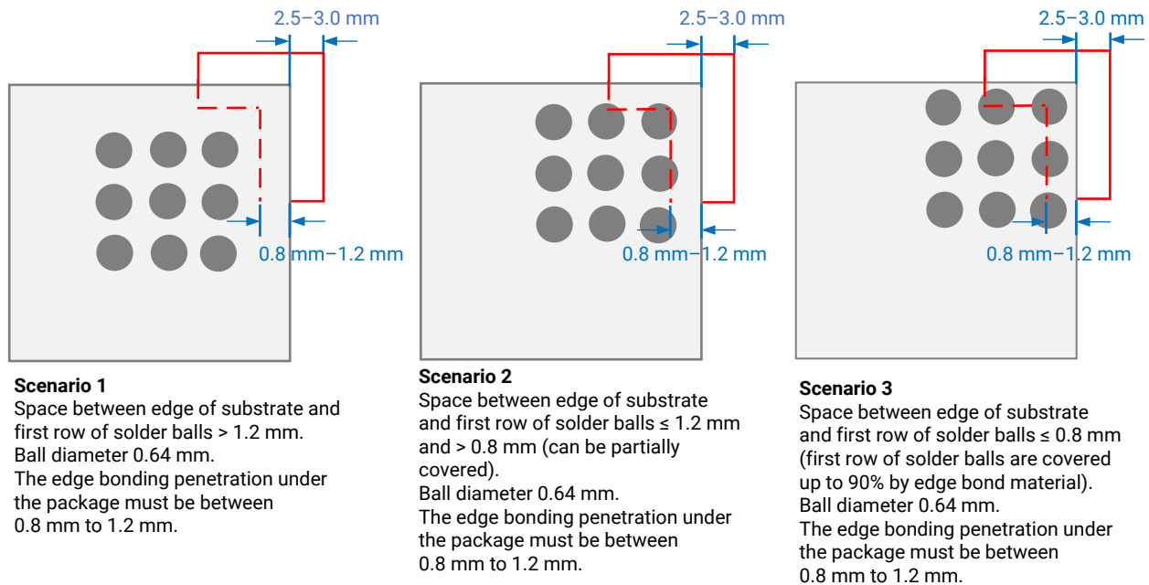
Figure 18: Edge Bonding Scenarios
