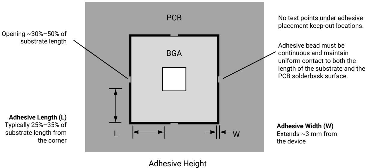
Figure 19: Edge Bonding Adhesive Placement Parameters
