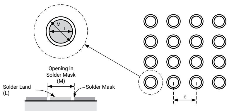
Figure 15: Suggested Board Layout of Soldered Pads for BGA Packages
