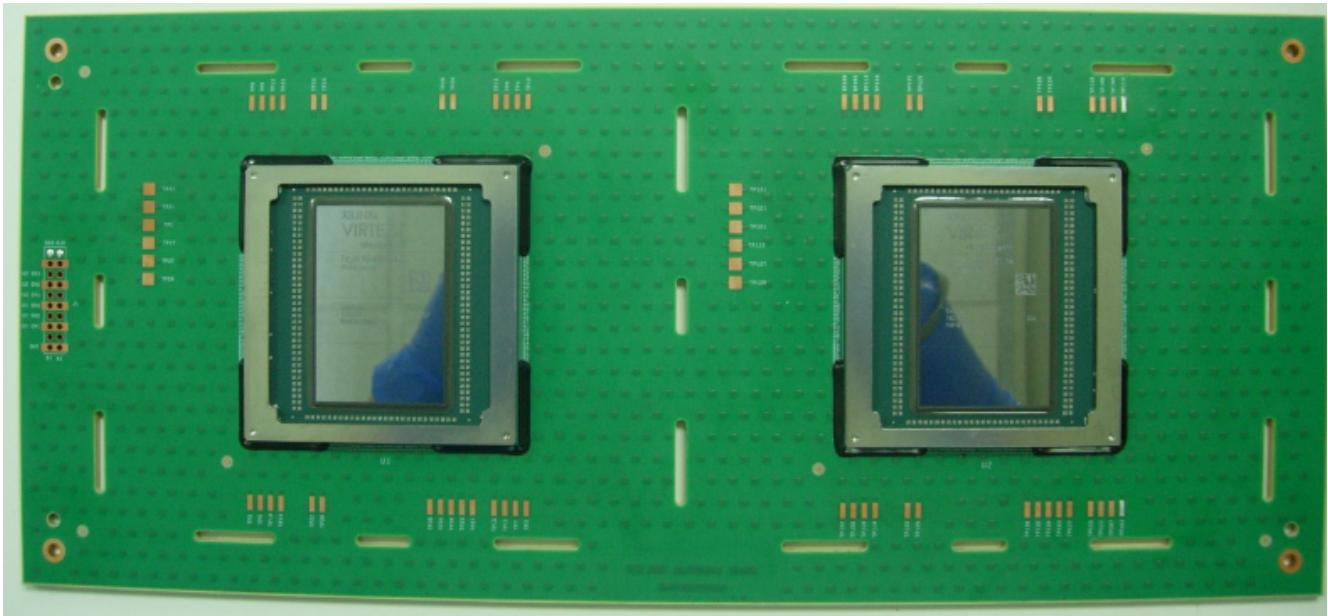
Figure 17: Edge Bonded BGA Packages
