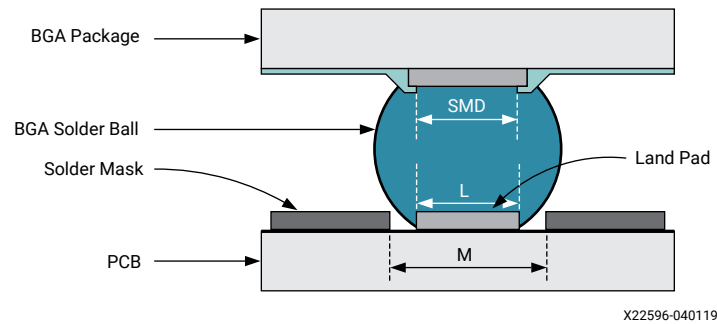
Figure 16: Example of an NSMD PCB Pad Solder Joint
