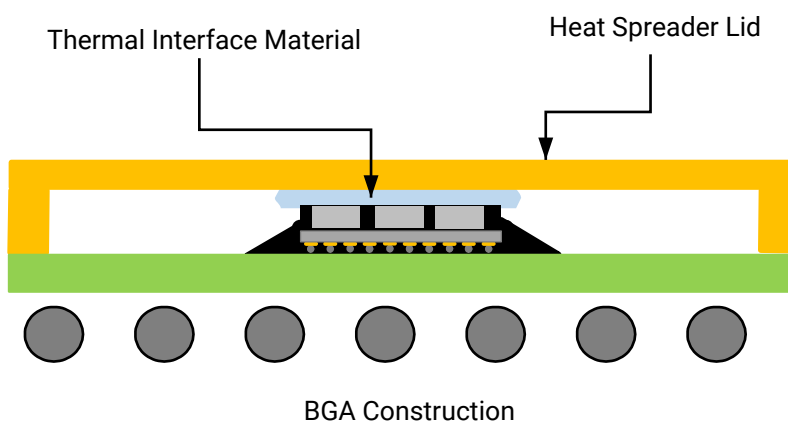
Figure 23: Lidded Flip-Chip BGA Construction with Heat Spreader and Thermal Interface Material
