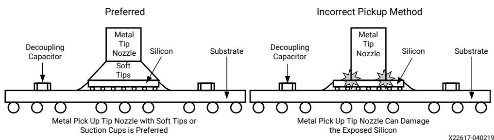
Figure 14: Recommended Method For Using Pick-up Tools
