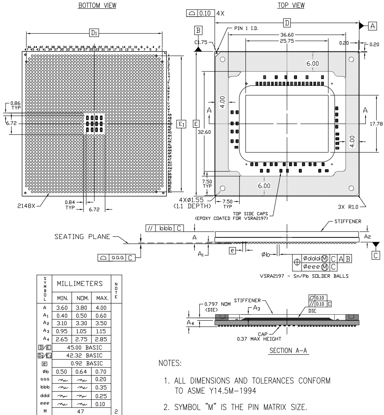
Figure 8: Package Dimensions for VSRA2197 (XQRVC1902)
