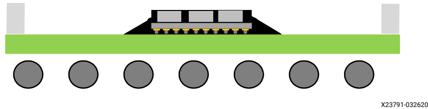
Figure 24: Lidless Flip-Chip BGA Construction
