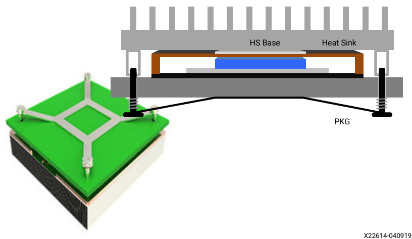
Figure 21: Dynamic Mounting and Bracket Clips on Heat Sink Attachment
