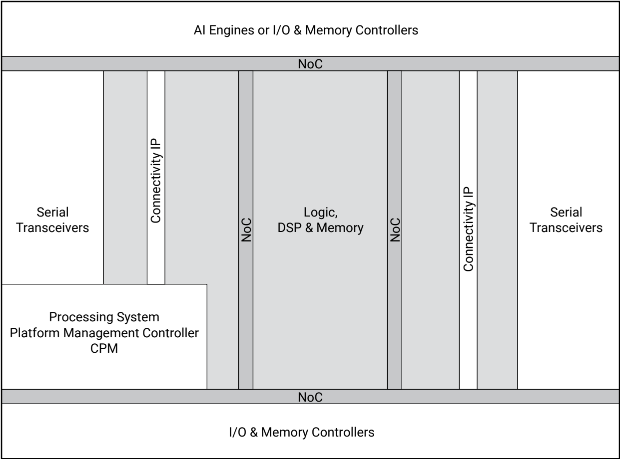
Figure 2: Versal AI Core XQR device Layout
