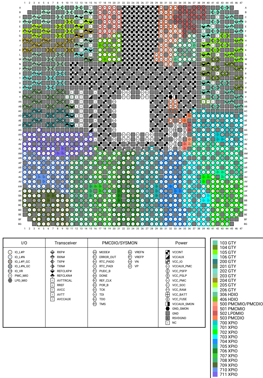
Figure 7: VSRA2197 Package—XQRVC1902 Device Diagram
