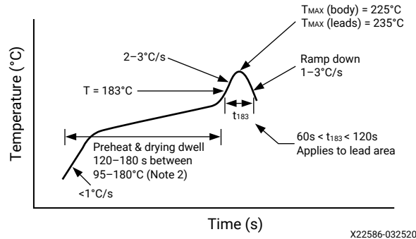
Figure 11: Typical Conditions for IR Reflow Soldering of Sn/Pb Solder
