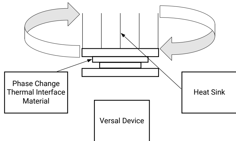
Figure 22: Breaking the Bond between Thermal Interface Material and Mated Components
